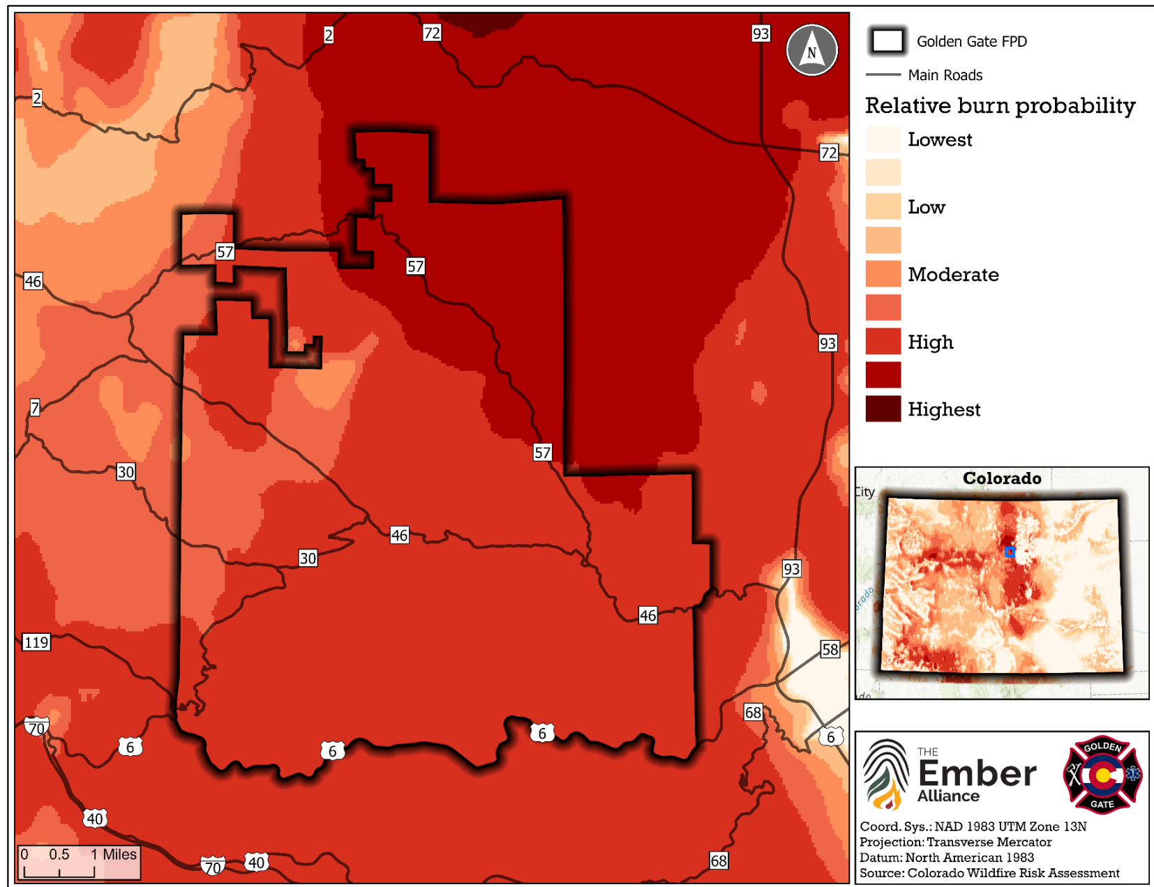
Figure B.7. Relative burn probability under various weather conditions compared to the rest of the state of Colorado. Source: 2022 CO-WRA.
