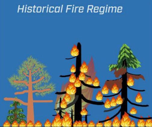
Figure 2.e.1. Fire behavior has changed for many ecosystems along the Front Range of Colorado, partially due to the suppression of wildfires for over a century. Source: Colorado Forest Restoration Institute..
